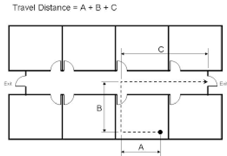
Travel Distance Calculation
