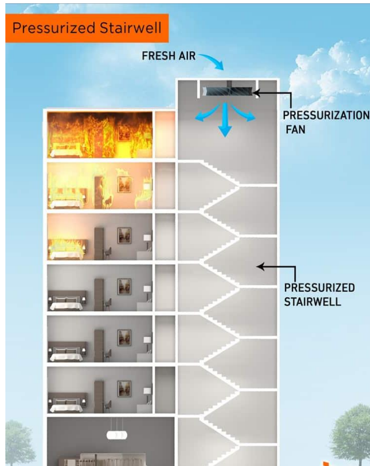
Staircase Pressurization System
