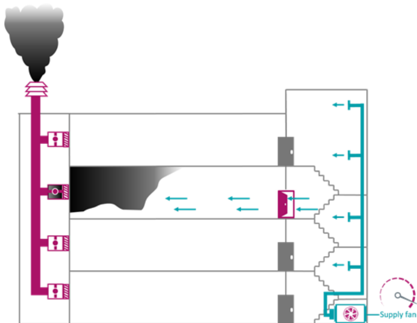
SmokeExhaust System
