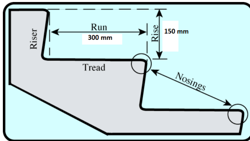
Riser and Tread of Staircase
