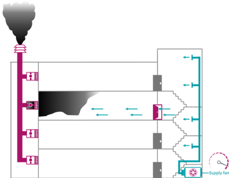
SmokeExhaust System
