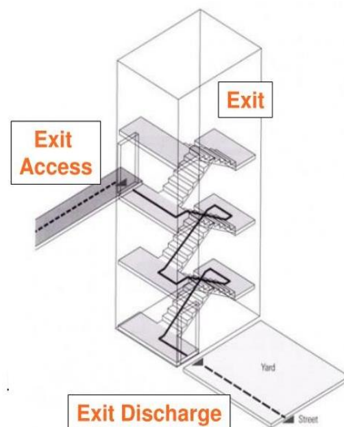
Figure 12: Means of Egress, Exit, Exit Discharge
