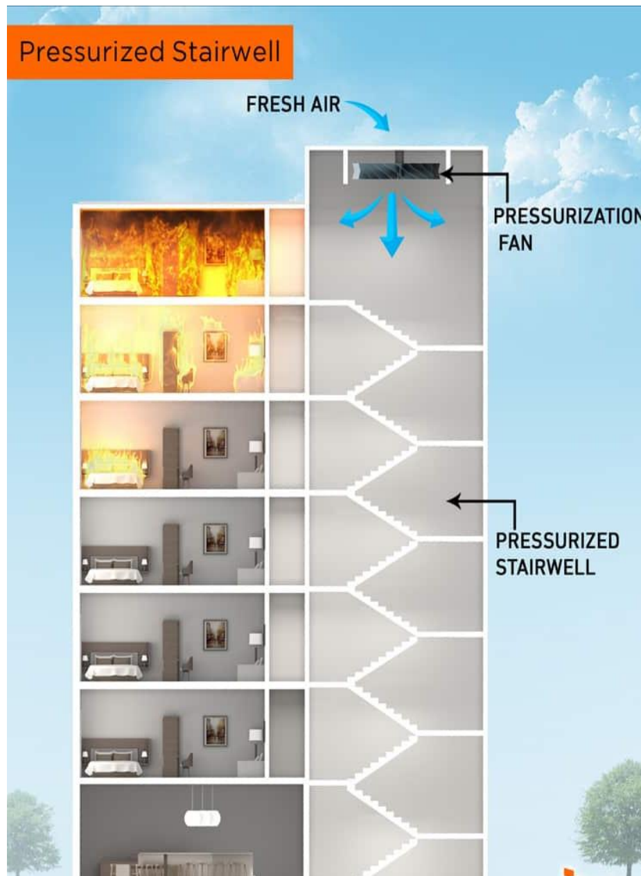
Staircase Pressurization System
