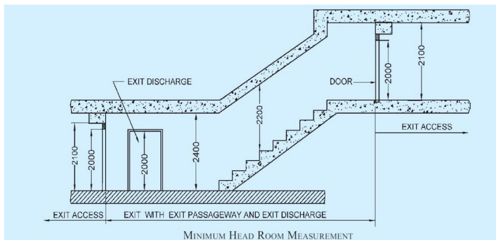
Exit Height
