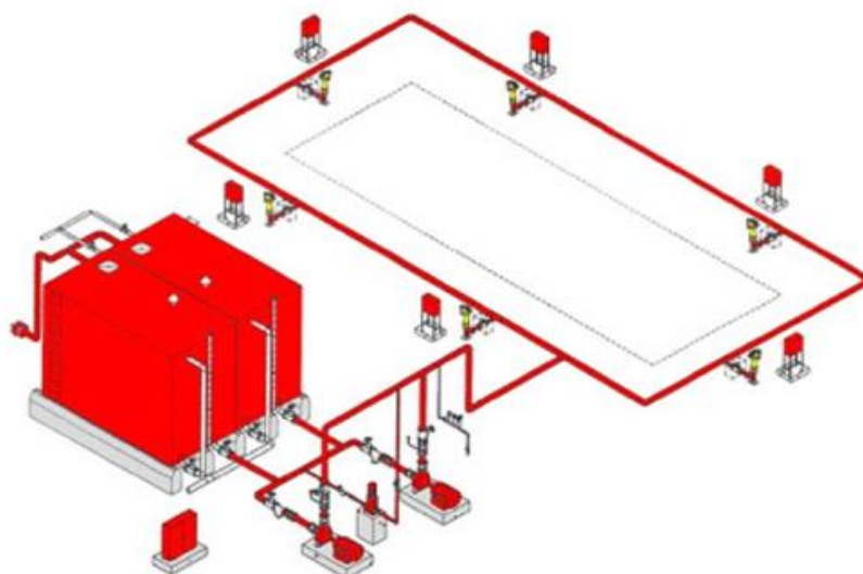
Yard hydrant picture
