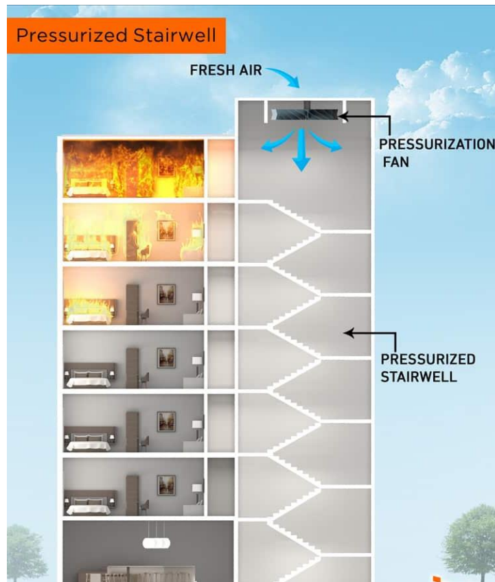
Staircase Pressurization System
