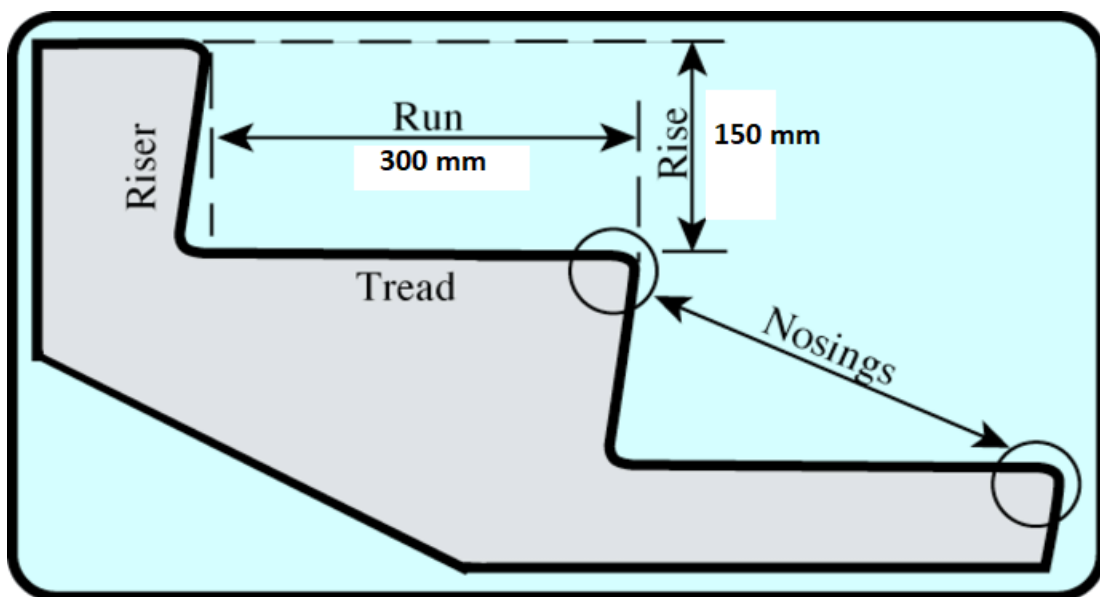
Riser and Tread of Staircase
