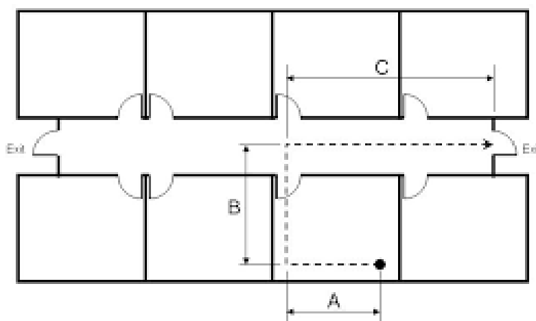
Travel Distance Calculation
