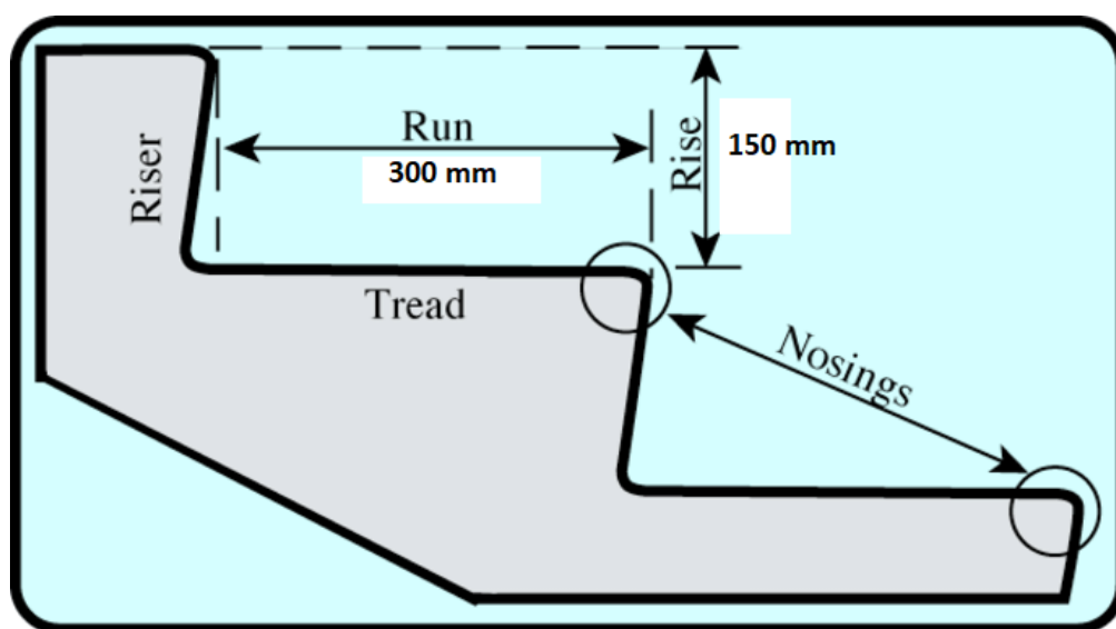
Riser and Tread of Staircase
